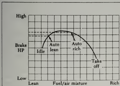
FIGURE 3-2. Power versus fuel/air mixture curve.
